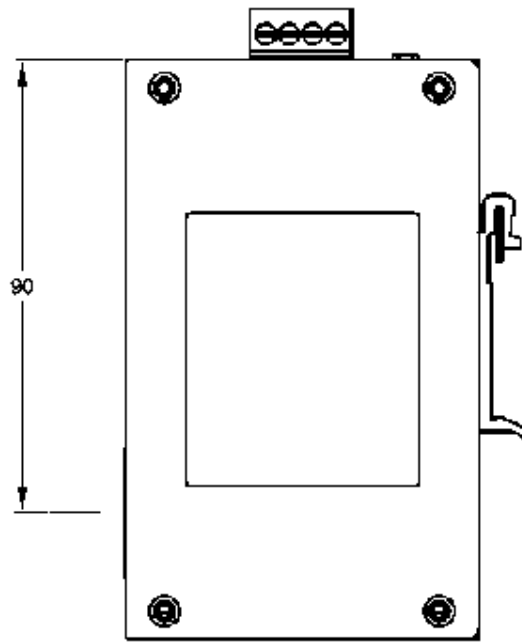
SC Fiber Models
